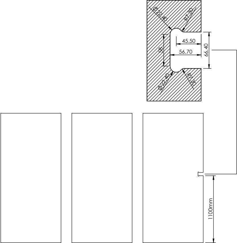
Hole Positon of Locks for Front Sliding Doors
